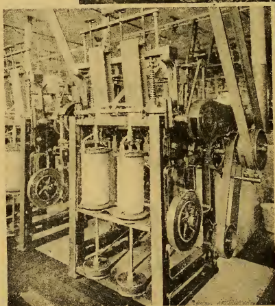
FINISHING BOX — ENGLISH DRAWING
